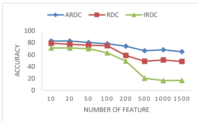
FIGURE 5. Accuracy comparison of ARDC, RDC and IRDC using Reuter21578 dataset and MLP.
