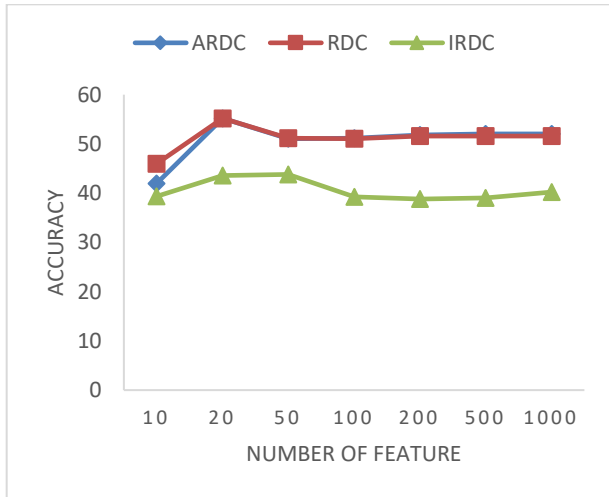
FIGURE 13. Accuracy comparison of ARDC, RDC and IRDC using TDT2 dataset and MNB.
