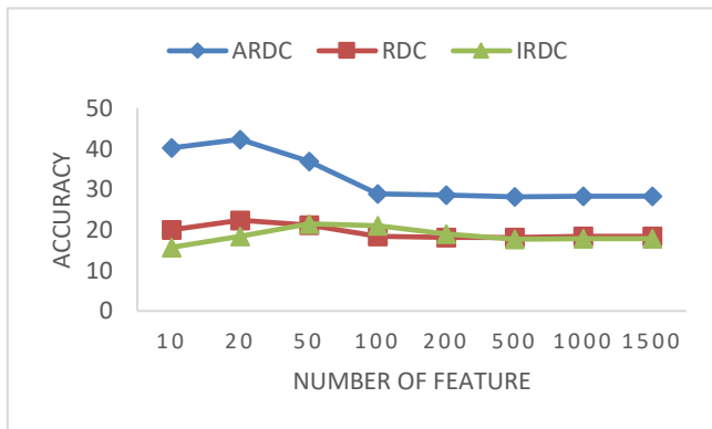
FIGURE 8. Accuracy comparison of ARDC, RDC and IRDC using 20newsgroup dataset and MNB.
