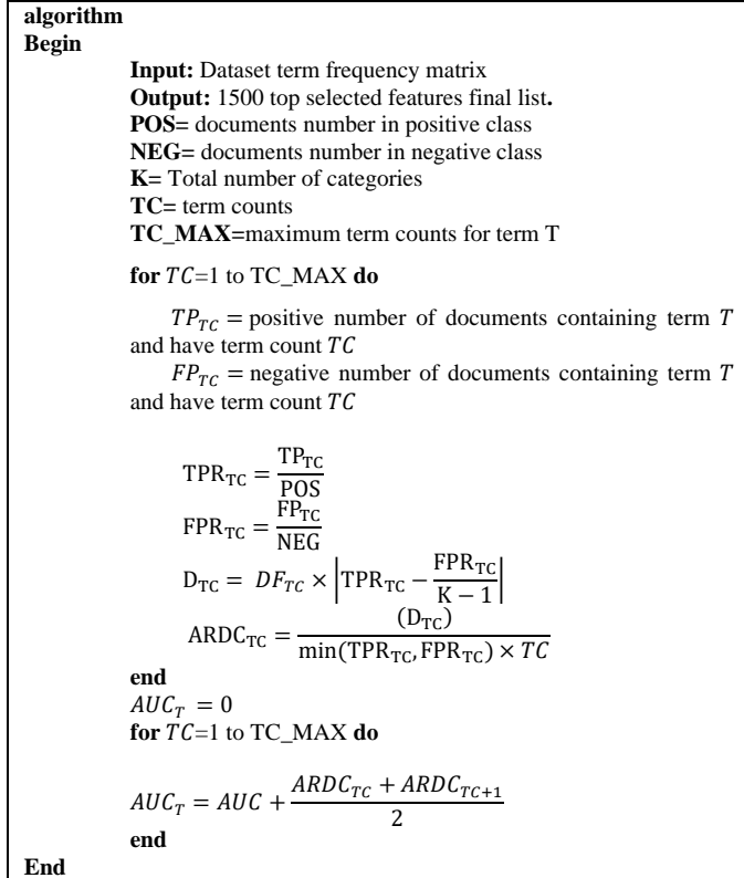
FIGURE 2. The algorithm of ARDC.
