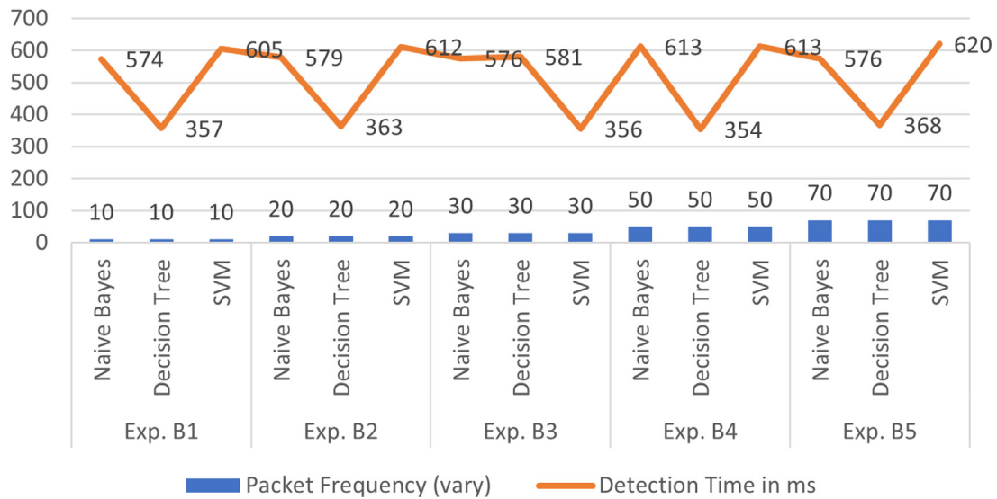
Fig. 8. Experiment B with IoT packet variations.
