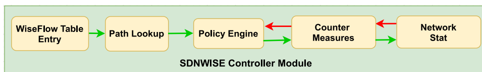
Fig. 4. SDN-WISE controller module.
