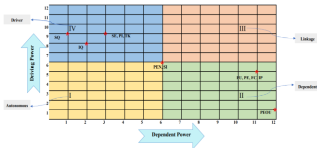
Fig. 6. MICMAC analysis
