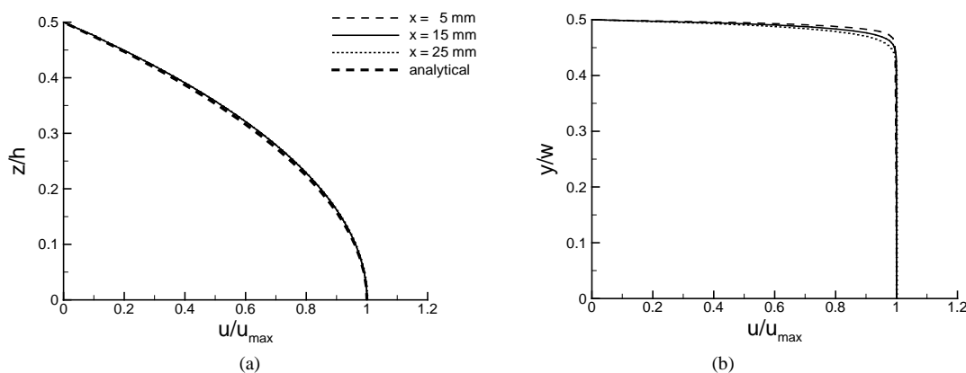
Figure 2. Velocity profiles at selected cross sections in the converging flow chamber. (a). Normalized profiles on the mid-width plane, i.e. y = 0 , together with the analytical solution; (b). Normalized velocity distribution on the mid-height plane, i.e. z = 0 . In the figure, L = 30 mm, w_0 = 10 mm, w_1 = 4 mm, h = 0.2 mm and Q = 1 ml/s.
