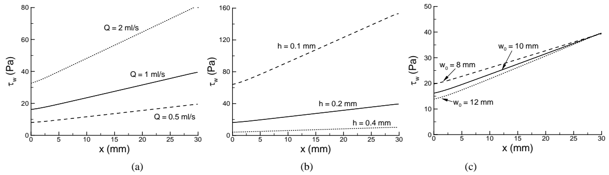
Figure 4. Effects of parameters on WSS and WSSG in the converging flow chamber. WSS distribution is plotted along the central line on the bottom/ top plate. Control parameters are L = 30 mm, w_0 = 10 mm, w_1 = 4 mm, h = 0.2 mm and Q = 1 ml/s. (a). Effect of Q ; (b) Effect of h ; (c) Effect of w_0 .
