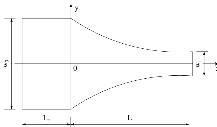
Figure 1. Schematic drawing of the converging parallel plate flow chamber. The length of the converging section is L . The width of the chamber, w , decreases from w_0 at the entrance to w_1 at the exit. A leading section of the length L_e and constant width w_0 is added at the entrance for inflow to become fully developed. The height of the chamber between the top and the bottom plates, h , is constant (not shown in the figure).
