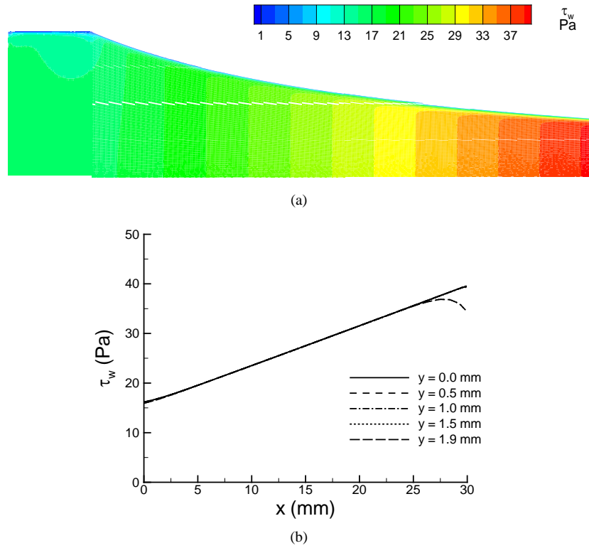
Figure 3. Wall shear stress distribution in the converging flow chamber. (a) WSS contours on the bottom/top plate; (b) Longitudinal profiles of WSS on the bottom/top plate. In the figure, L = 30 mm, w_0 = 10 mm, w_1 = 4 mm, h = 0.2 mm and Q = 1 ml/s.
