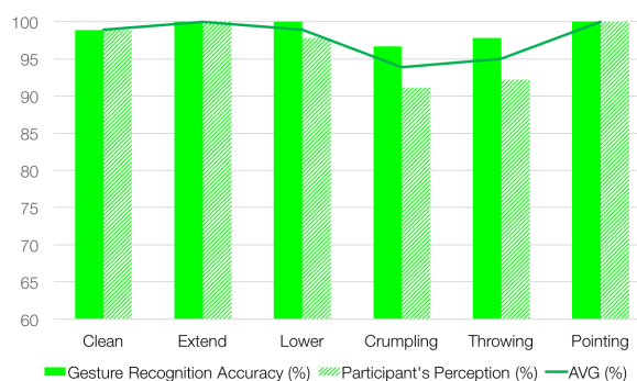
Figure 3: Usability study outcome.
