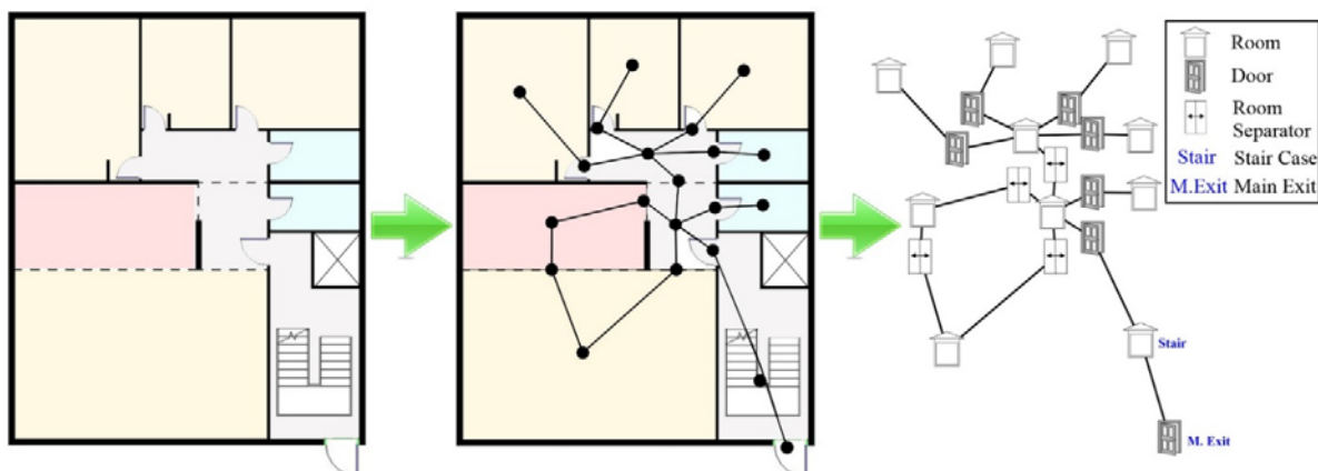
Figure 6. Process of graph extraction from BIM by the developed plugin.
