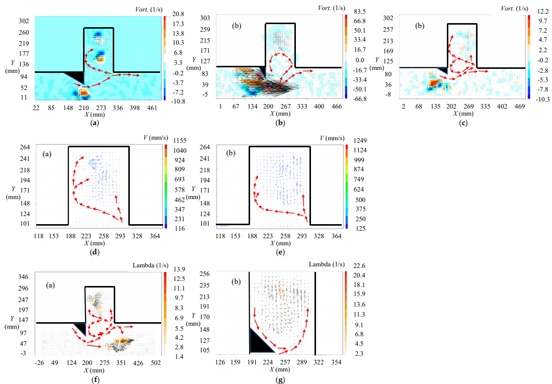
Figure 2. Observation of the flow field at the dead-end with different parameters of the spoiler using PIV: (a) With spoiler No. 2; (b) With spoiler No. 3; (c) With spoiler No. 4; (d) With spoiler No. 5; (e) With spoiler No. 6; (f) With spoiler No. 1 at the front edge of the main pipe; (g) With spoiler No. 1 at the entrance of the dead-end branch.
