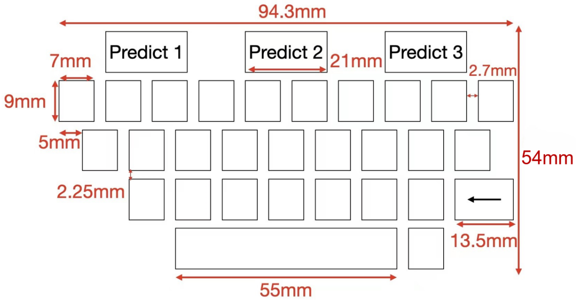
Fig. 4. OnArmQWERTY keyboard dimensions.
