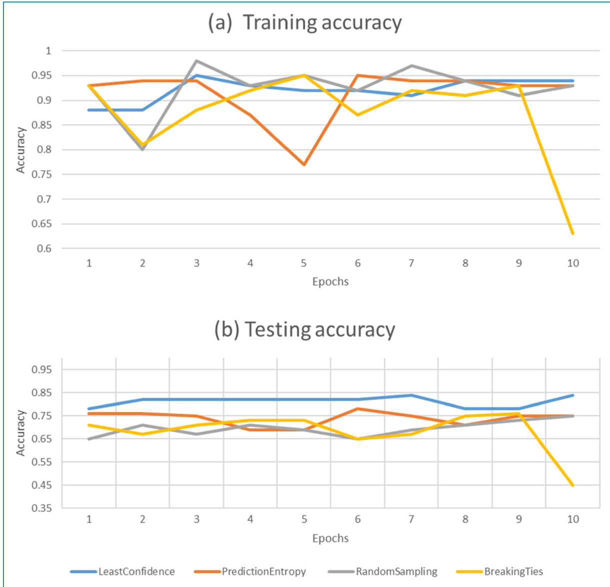
Figure 5. Performance of AL on annotations using different AL query strategies.
