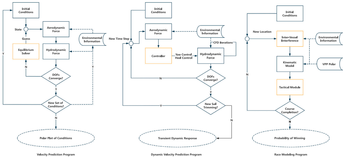
Fig. 5. Flowchart of the three performance evaluation frameworks.
