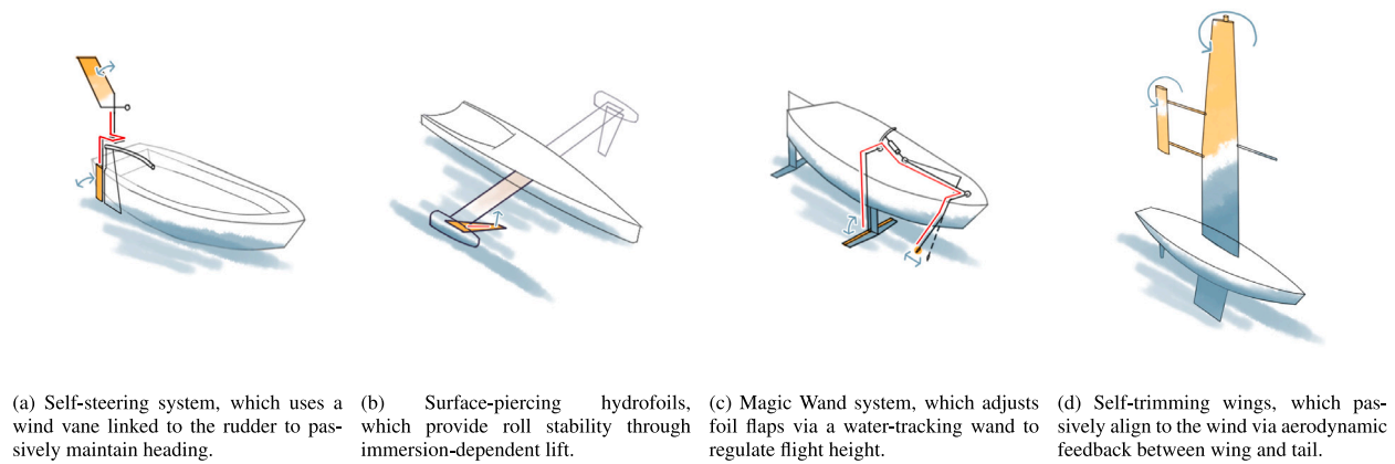
Fig. 7. Mechanical control systems in sailboats.
