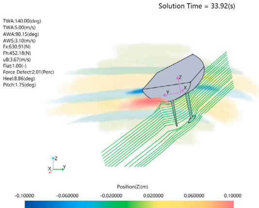
(b) CFD simulation of wave patterns under a specific test configuration, adapted from [83]
