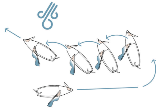
(b) Heaving-to stabilizes the boat with opposing sail and rudder forces, adapted from [225].
