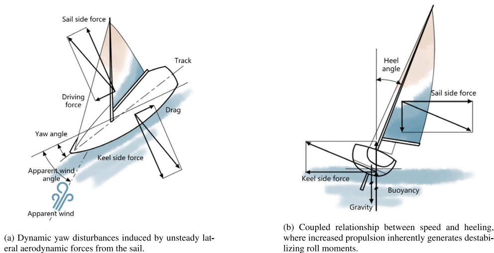
Fig. 6. Motion control challenges in sailing, adapted from [141].
