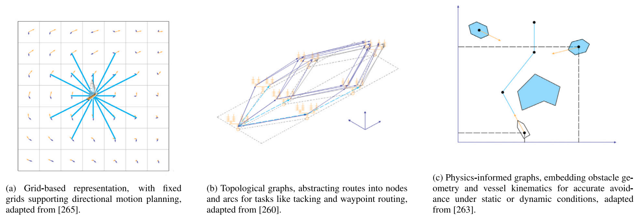
Fig. 10. Environmental modeling methods for sailboat navigation (see [260,263,265]).
